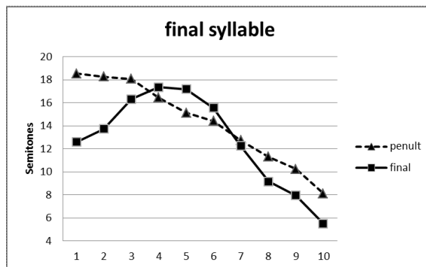
Figure 6: F0 (in semitones) measured at ten intervals through the final foot (CV.CV or CVC).
