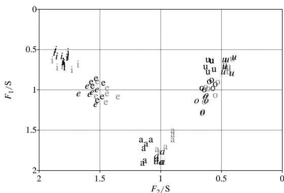
Figure 6: F1/S~F2/S plot of Spanish vowels: nanny (black), Sofia (grey) and Maya (italics).
