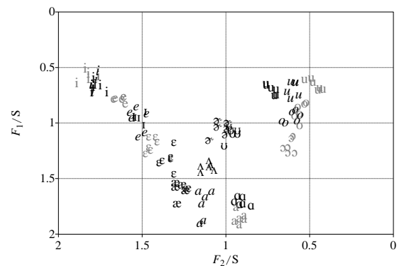
Figure 1: F1/S~F2/S plot of adult vowels in English (black), Italian (grey) and Spanish (italics).
