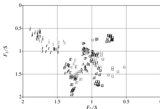
Figure 4: F1/S~F2/S plot of English vowels: father (black), Sofia (grey) and Maya (italics).
