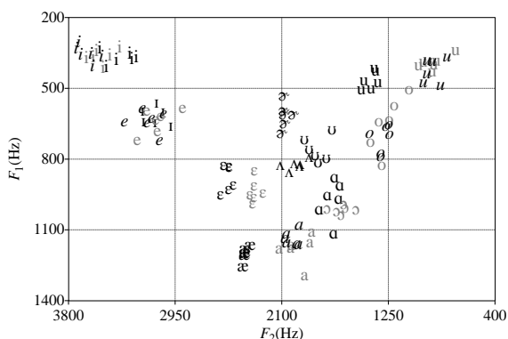
Figure 3: F1~F2 plot of Maya's vowels in English (black), Italian (grey) and Spanish (italics).
