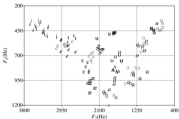
Figure 2: F1~F2 plot of Sofia's vowels in English (black), Italian (grey) and Spanish (italics).
