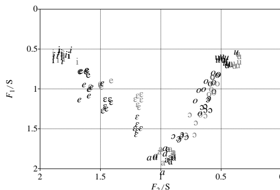
Figure 5: F1/S~F2/S plot of Italian vowels: mother (black), Sofia (grey) and Maya (italics).
