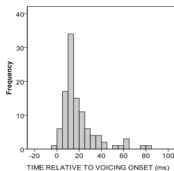
Figure 3: Frequency distribution of onset of nasal closure relative to phonation onset (time 0) in Spanish prenasalized voiced stops. N= 107.
