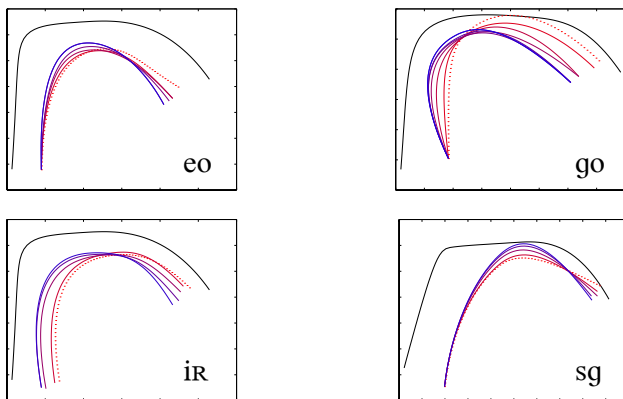
Figure 7: Pivots for [eo], [go], [iR], [sg].
