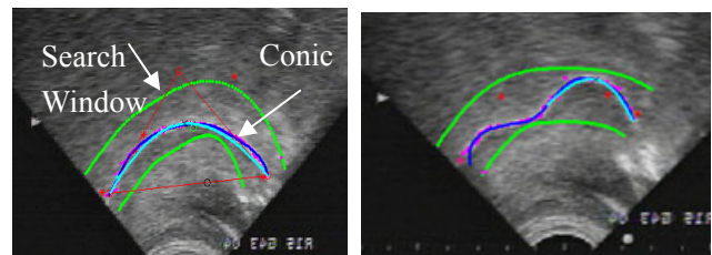
Figure 6: a) Conic fit for entire tongue for [ə]. b) 3 Conic fit for American English [r].
