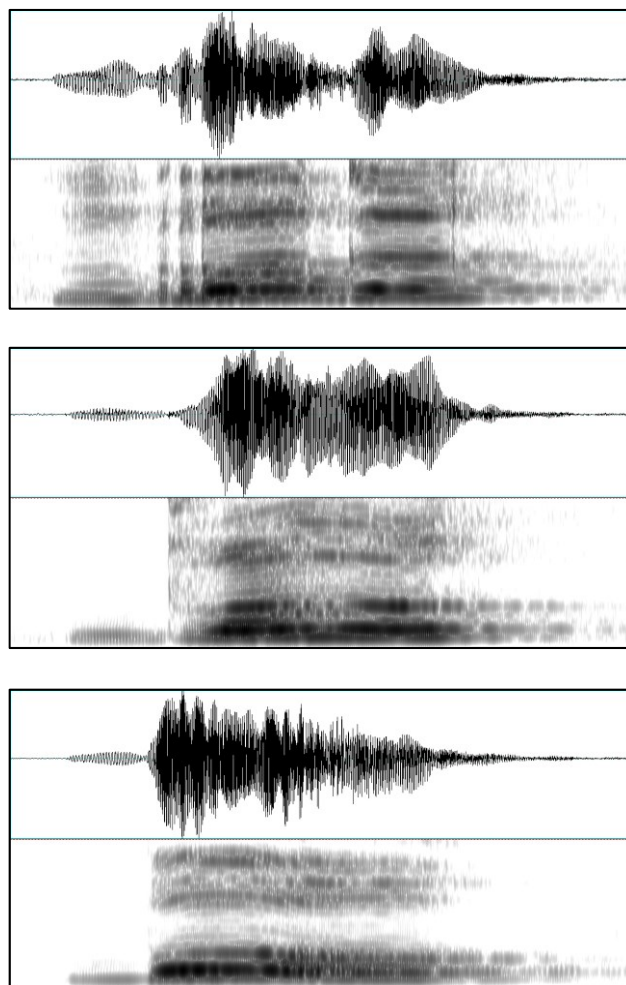
Figure 1: Waveforms and spectrograms of [mbʰóǵ] ‘fire’, [bʰβóǵ] ‘poverty’, and [bʰò] ‘two’.
